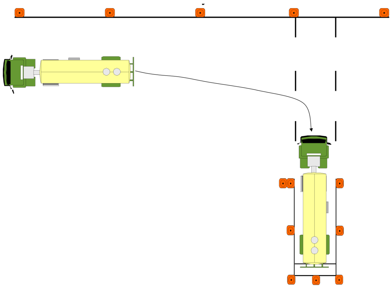
Figure 11.6: Alley Dock
